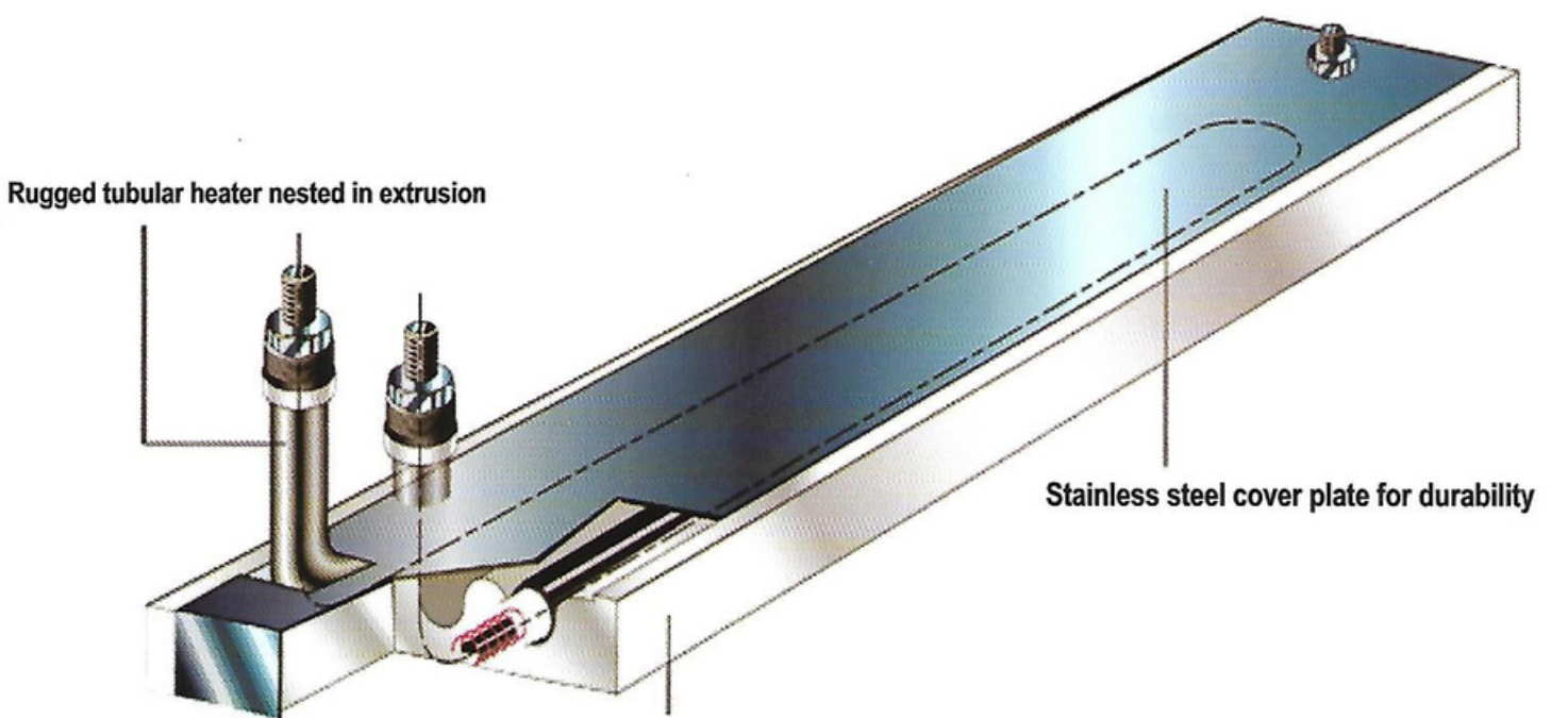
Extruded aluminum serves as an excellent heat transfer medium
